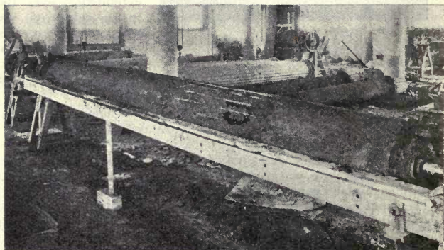
FIG. 50—MAKING HOLLOW REINFORCED CONCRETE COLUMN BY MEANS OF MANDREL
